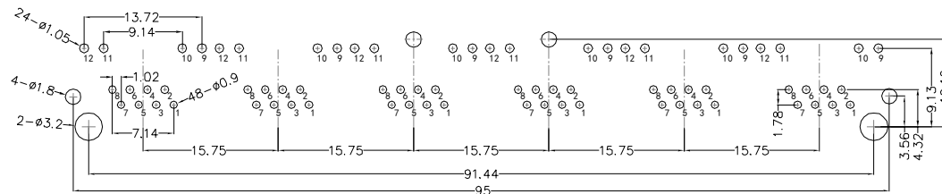
RECOMMENDED PCB LAYOUT VIEWED FROM COMPONENT SIDE
